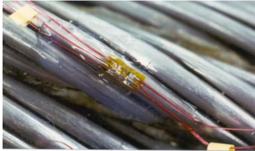
Rosette 3 directions
